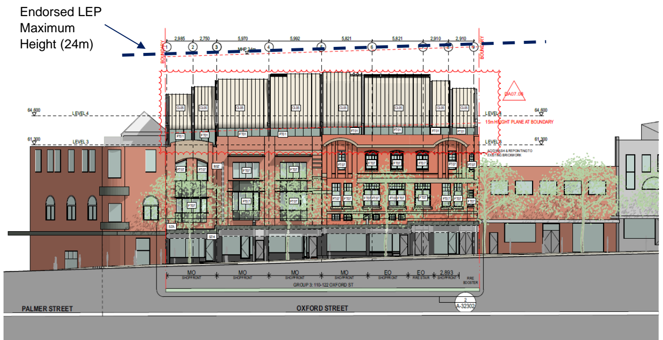
Figure 4 Proposed new addition and the 15m height plane
